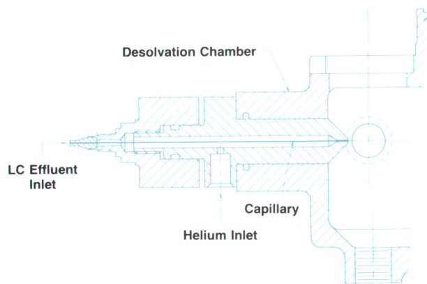
Fig. 3. Nebulizer detail.
