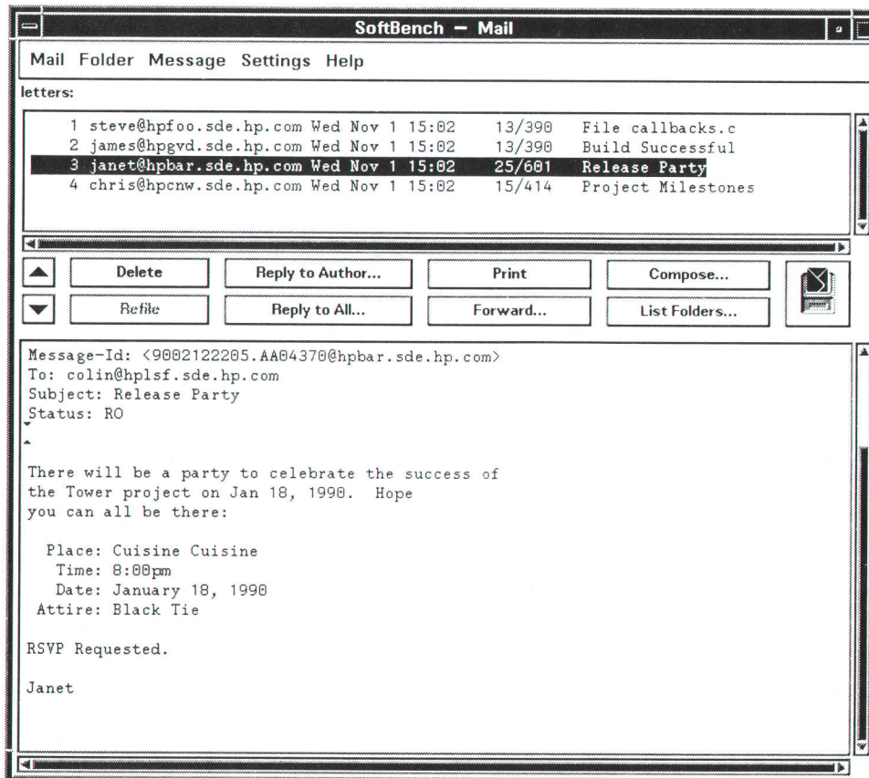
Fig. 2. User interface of the HP SoftBench mail tool, an encapsulation of mailx .
