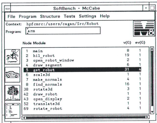
Fig. 4. Encapsulation of the Analysis of Complexity Tool (ACT) from McCabe and Associates.
