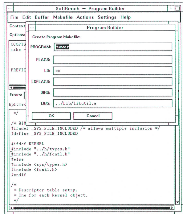
Fig. 2. Creating a makefile in the program builder.
