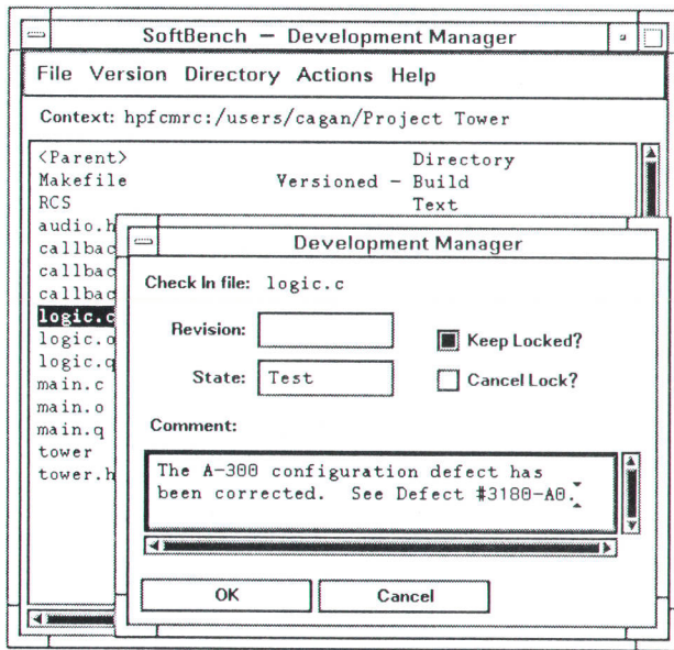
Fig. 3. An example of a dialog box prompting the user for version information.
