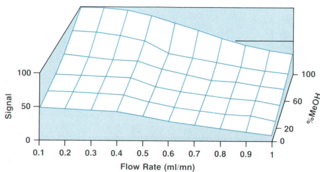
Fig. 7. Effects on sensitivity of mobile phase flow rate and composition.
