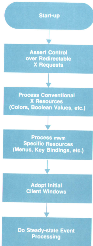
Fig. 3. OSF/Motif Window Manager start-up process.
