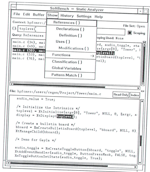
Fig. 1. Static analyzer user interface.
