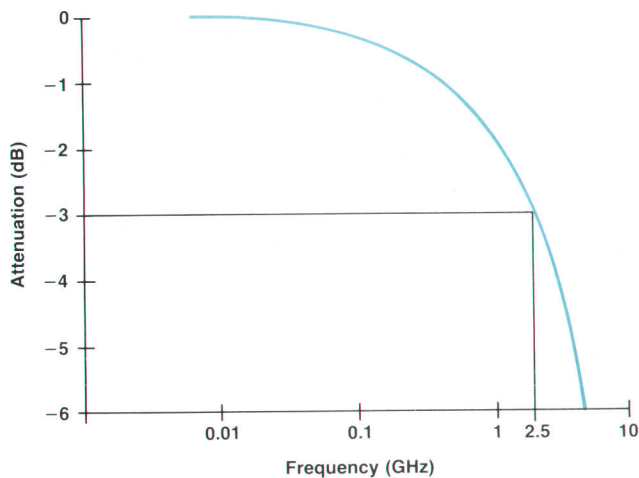
Fig. 10. Bode plot and the 3-dB bandwidth.
