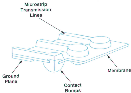
Fig. 5. The membrane probe concept.
