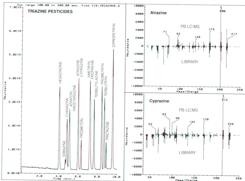
Fig. 11. Analysis of triazine pesticides by particle beam LC/MS.
