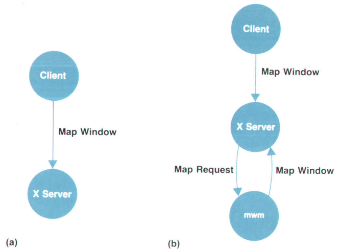
Fig. 4. Event redirection. (a) If no window manager is running (no redirection), the client's window mapping is done immediately. (b) When mwm is running, the server redirects the client's map window request to mwm. Mwm adds its window border before asking the server to complete the window mapping.
