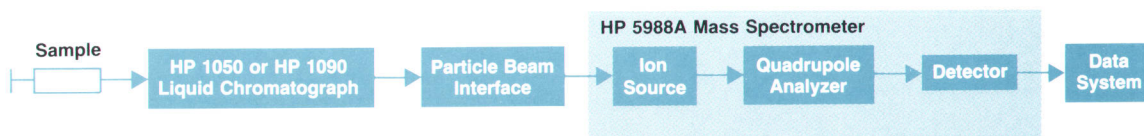
Fig. 1. For particle beam liquid chromatography/mass spectrometry (LC/MS), a special interface is mounted between the LC and MS systems. The data system can be either an HP 59970C ChemStation for single-instrument operation or an HP 1000 computer system for multiinstrument, multitasking, multiuser operation.
