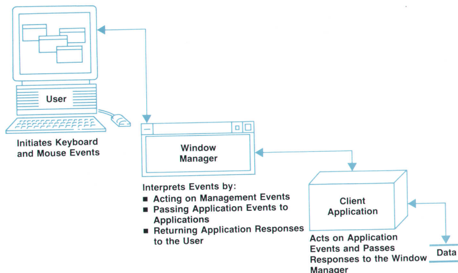
Fig. 1. Interactions between some of the components in the OSF/Motif hierarchy.
