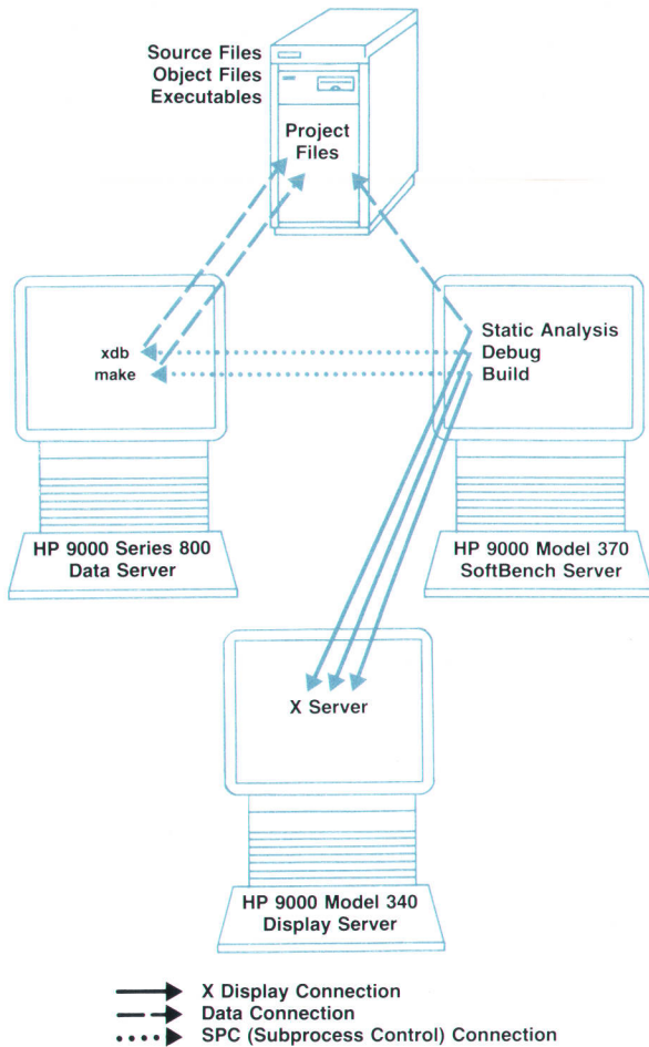
Fig. 1. An example of an HP SoftBench distributed development environment.
