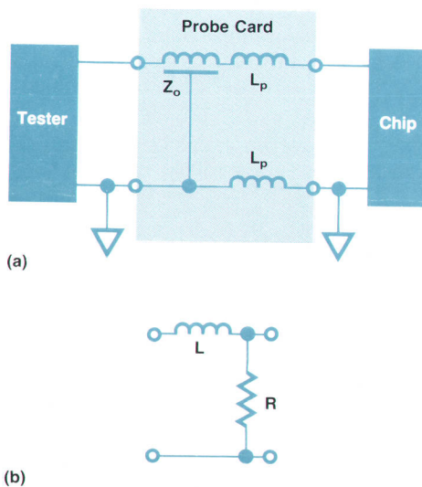
Fig. 2. The conventional probe as a signal line. (a) Equivalent circuit. (b) Equivalent low-pass filter.
