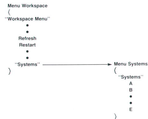
Fig. 11. The Systems menu is cascaded from the Workspace menu because of the entry in Workspace that calls the Systems menu.
