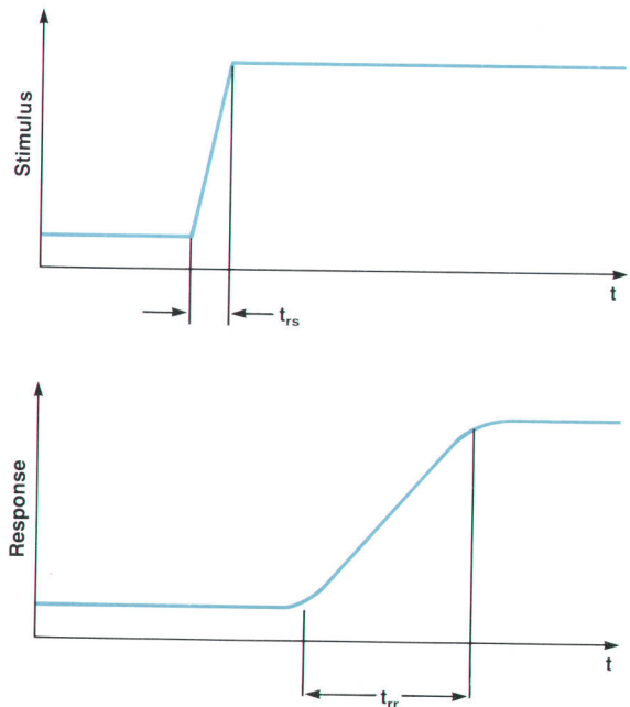
Fig. 3. The effect of parasitic inductance in the time domain.
