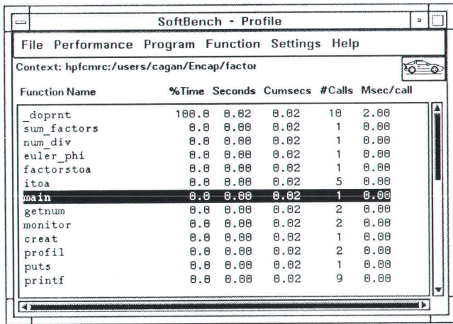
Fig. 3. Encapsulation of the HP-UX performance profiling tool prof.
