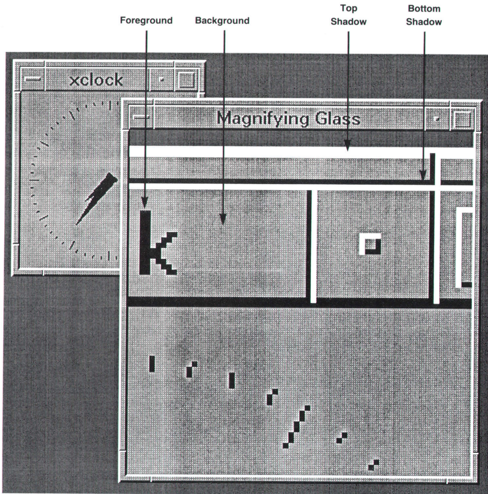
Fig. 12. The four colors involved in achieving the 3D look for a frame.
