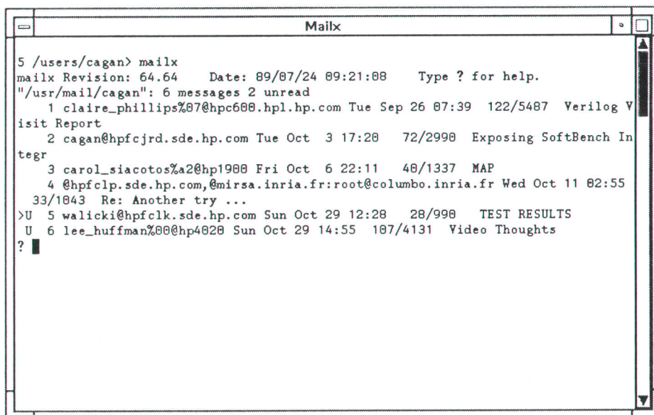
Fig. 1. Original user interface of the HP-UX terminal-based mail tool mailx.
