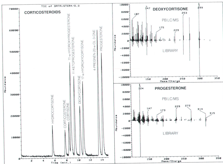
Fig. 12. Separation of corticosteroids by particle beam LC/MS.
