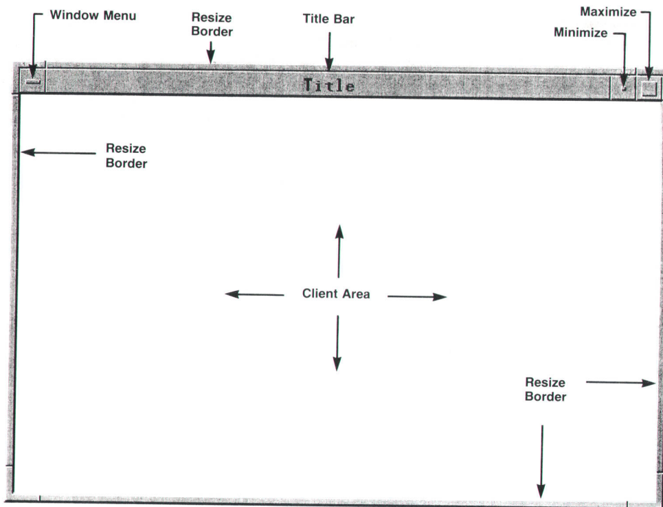
Fig. 3. The frame of a window in the OSF/Motif environment.
