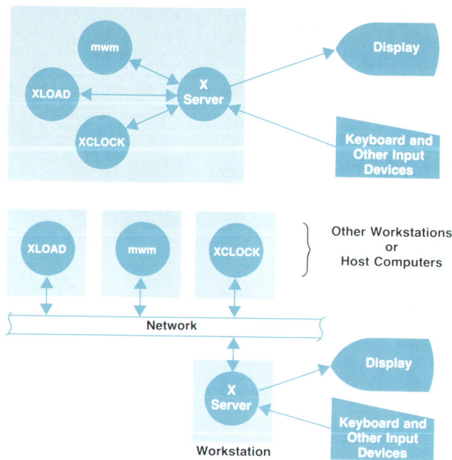
Fig. 1. The X client-server model. In this model the X server is near the user and controls the display and manages the input devices. The clients in this model are the applications that talk to the server using the X protocol, such as mwm, XLOAD, and XCLOCK. The X protocol allows the clients and server to run either on the same machine or on different machines connected by a network. (a) X client-server architecture on stand-alone workstation. (b) X client-server relationships in a distributed environment.
