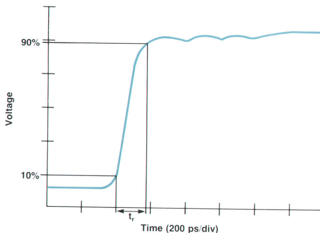
Fig. 9. Transmission response and rise time.
