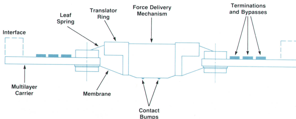
Fig. 6. Architecture of the membrane probe card.
