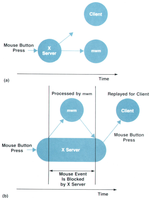
Fig. 10. (a) Mouse input stolen by mwm using a passive grab. The short arrow indicates that the button event never makes it to the client. (b) Mouse input intercepted by mwm and replayed.
