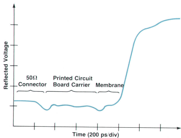
Fig. 8. Time-domain reflectometry profile and characteristic impedance.
