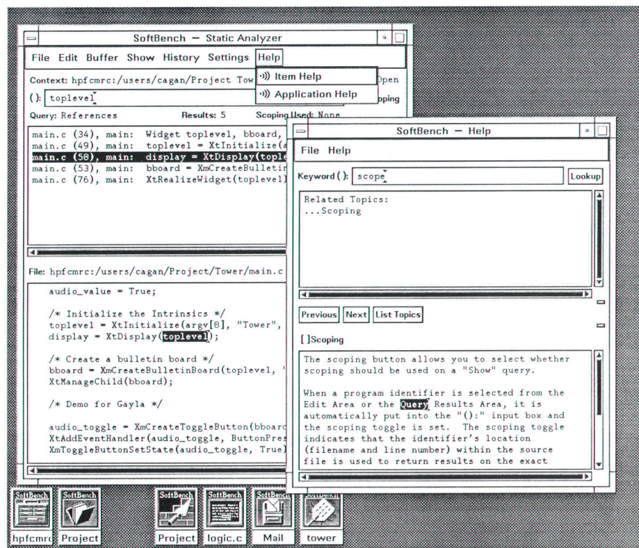
Fig. 1. HP SoftBench on-line help.
