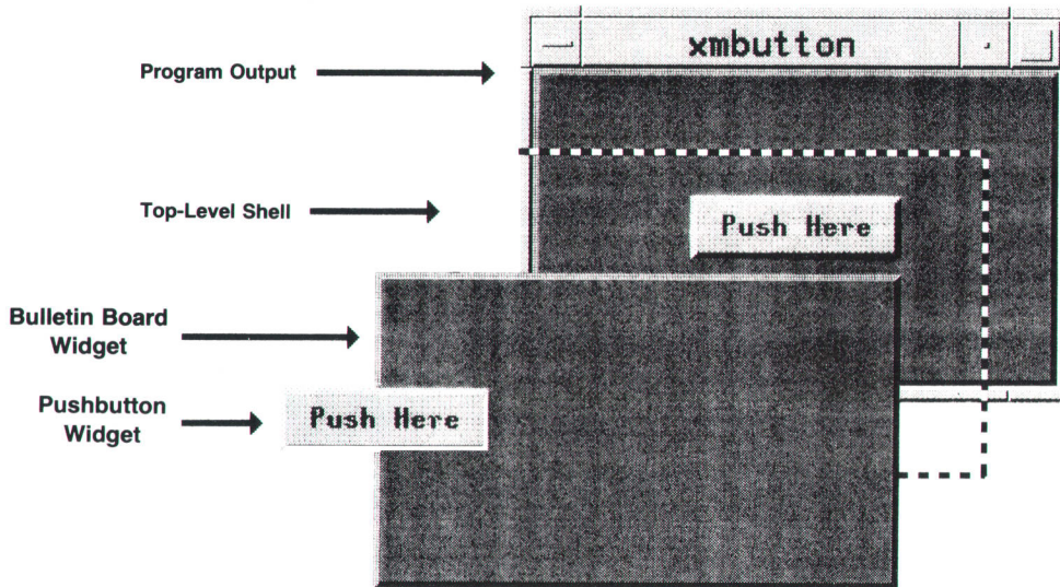
Fig. 2. Exploded view of widgets in a program.
