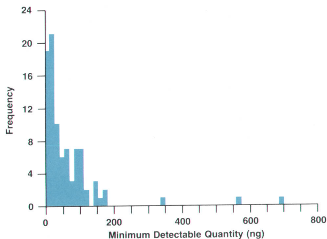
Fig. 8. Minimum detectable quantities for 92 pesticides for a signal-to-noise ratio of 2 in full-scan data acquisition.
