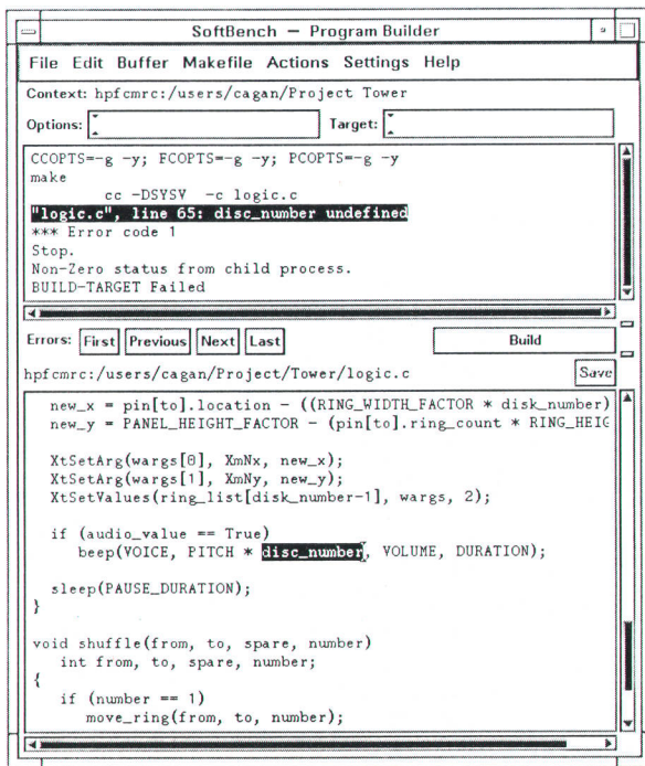
Fig. 1. Program builder user interface.
