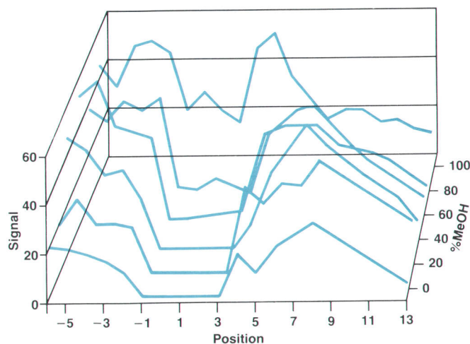
Fig. 4. Signal intensity for 10-ng injections of caffeine as a function of nebulizer position and mobile phase.
