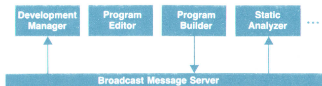
Fig. 2. HP SoftBench tools communicate through the broadcast message server. Tools receive only messages they want to receive.
