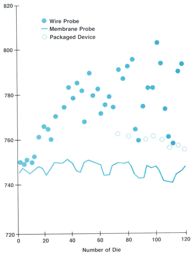
Fig. 12. Measurement accuracy.
