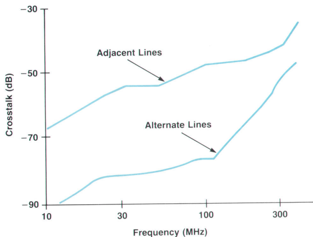
Fig. 11. Cross talk.
