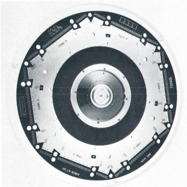
Fig. 16. The membrane probe for microprocessor testing.
