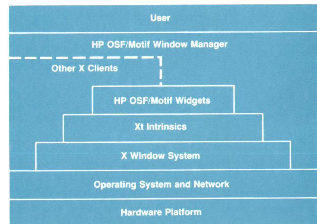
Fig. 1. The X Window System and other components in the OSF/Motif environment. The dashed line indicates that other X clients can either be managed by the window manager or run independently of the window manager.
