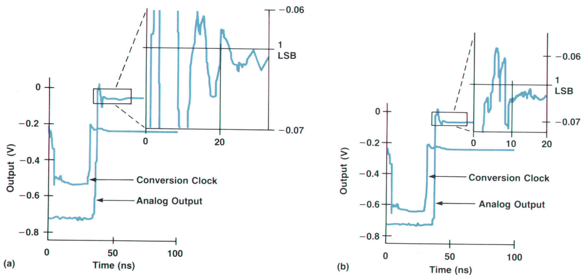
Fig. 15. Settling time of the DAC analog output. (a) Conventional probe card. (b) Membrane probe card
