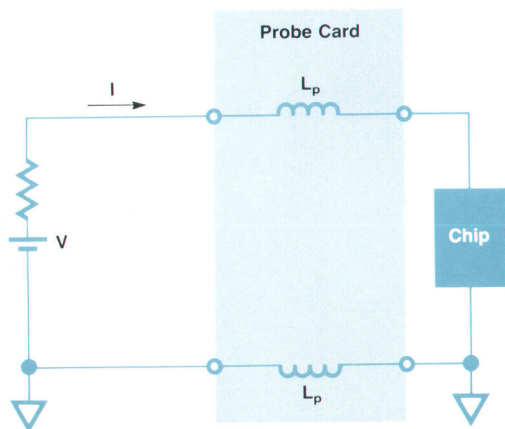
Fig. 4. A power line in a conventional probe.
