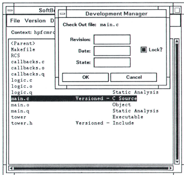
Fig. 1. Development manager user interface.
