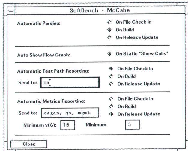
Fig. 5. Triggers for the encapsulation of McCabe's ACT.
