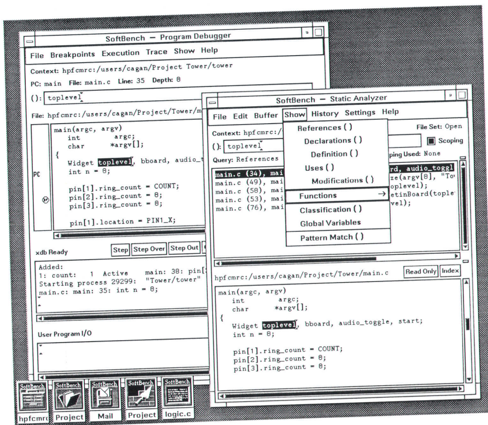
Fig. 1. Typical HP SoftBench user interface.
