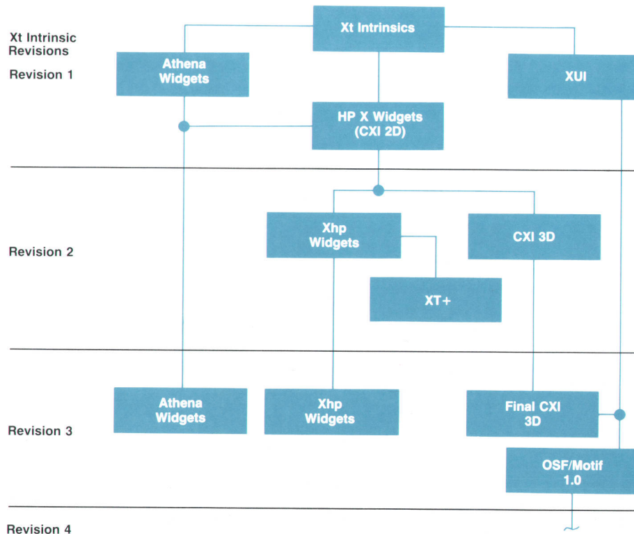
Fig. 1. The widget family tree. Different improved versions of the Xt Intrinsic were used to implement different versions of the widget family.
