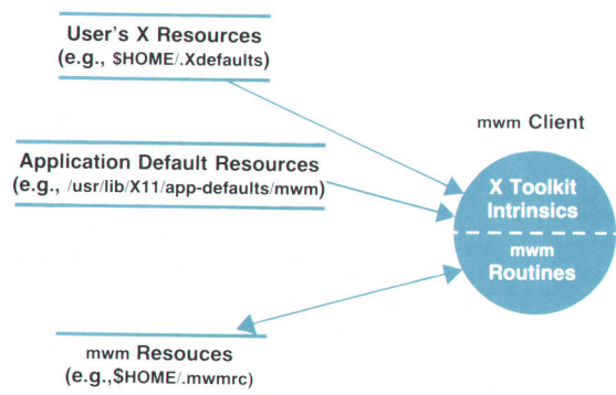
Fig. 5. Resource files used by mwm.
