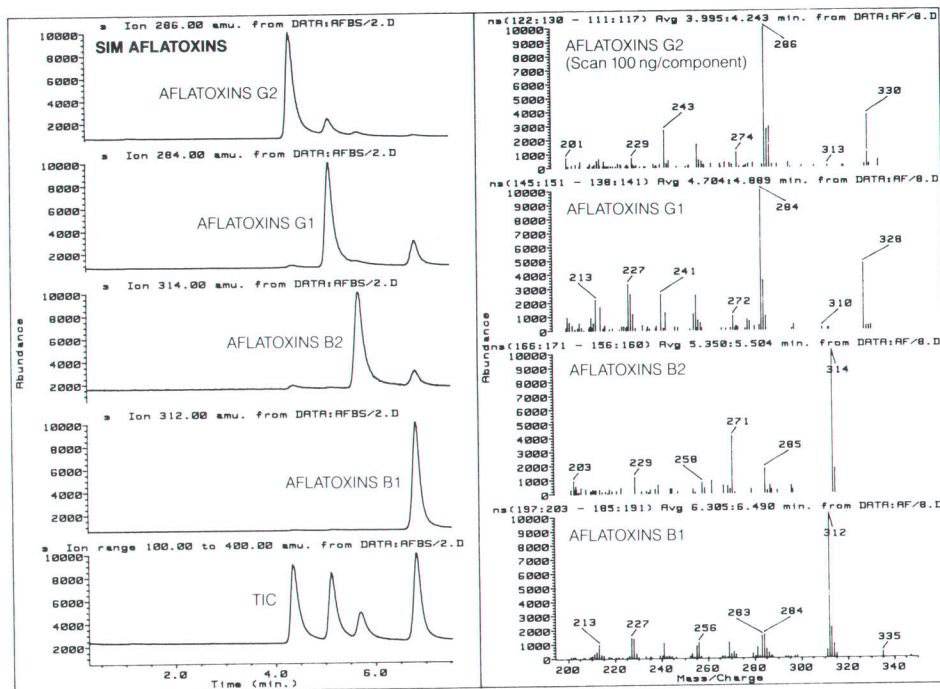
Fig. 13. Separation of aflatoxins by particle beam LC/MS.
