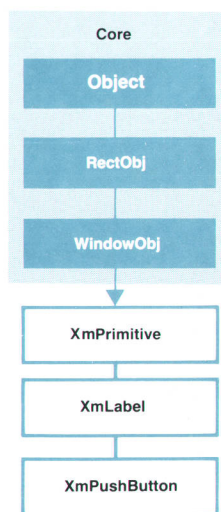
Fig. 3. Basic widget hierarchy.
