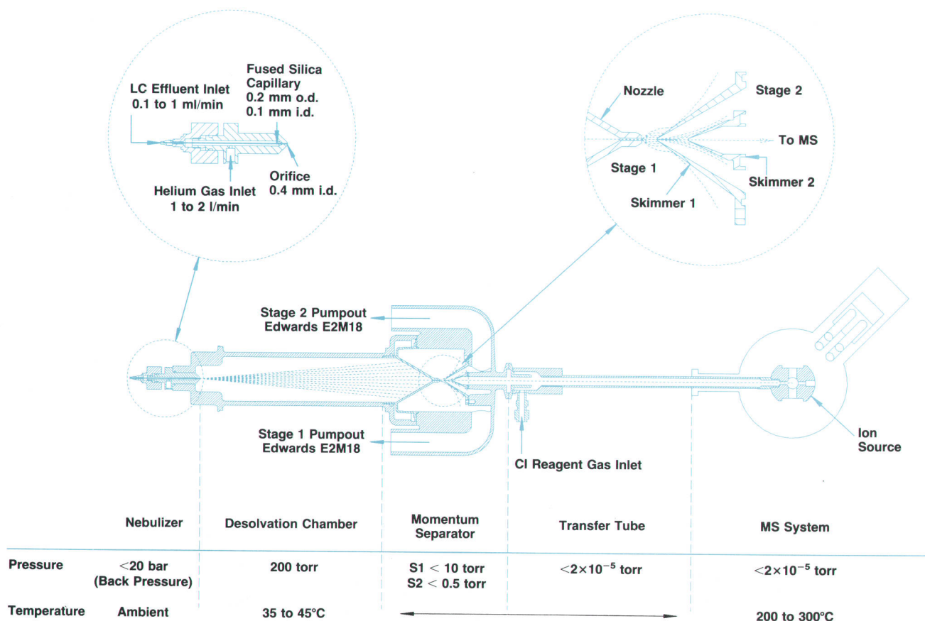
Fig. 2. Diagram of the HP particle beam interface for LC/MS.
