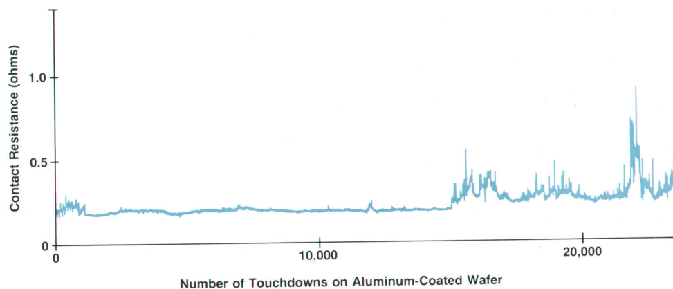
Fig. 7. Contact resistance as a function of the number of touchdowns.
