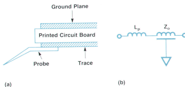
Fig. 1. Conventional wafer probe. (a) Structure. (b) Equivalent circuit.
