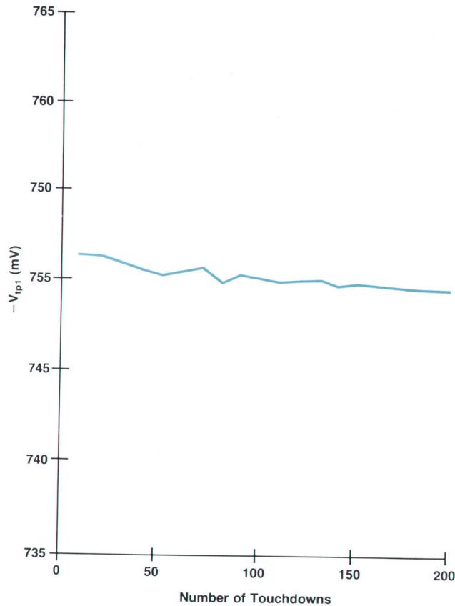
Fig. 13. Measurement repeatability.
