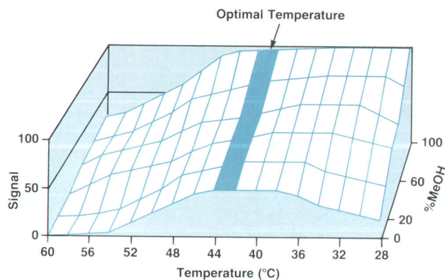
Fig. 5. Effects on sensitivity of desolvation chamber temperature and mobile phase composition.
