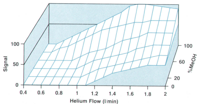
Fig. 6. Effects on sensitivity of mobile phase composition and helium flow rate.
